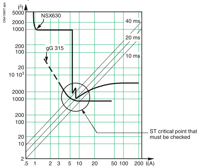
I²t curve for Compact NSX and a fuse.
