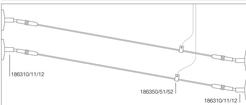
Cable system wall-to-wall installation scheme (walls NOT perpendicular to the cable system)
