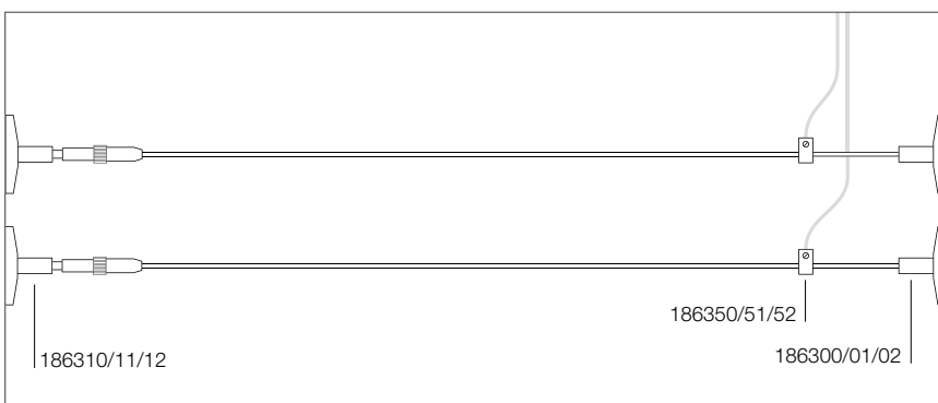
Cable system wall-to-wall installation scheme, no cable tensioner (perpendicular to wall)
