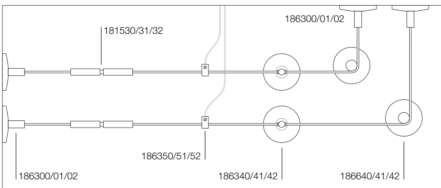
Cable system wall-to-wall installation scheme, with changing in direction
