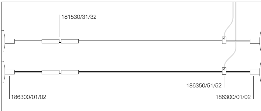
Cable system, wall-to-wall installation scheme (perpendicular to wall)
