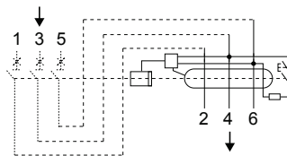
Wiring diagram
