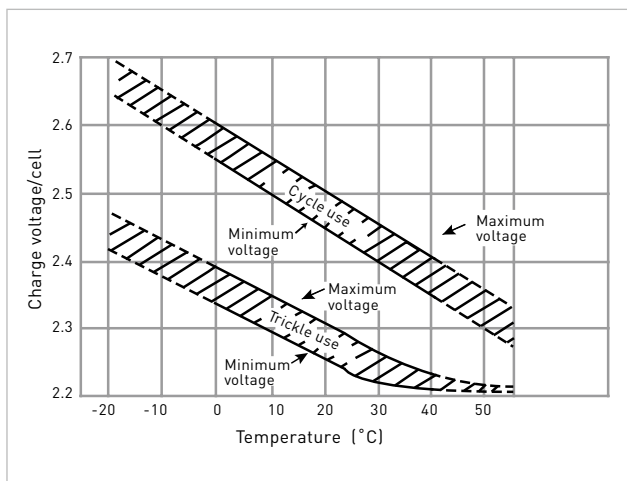
Fig. 6 Compensated voltage value
