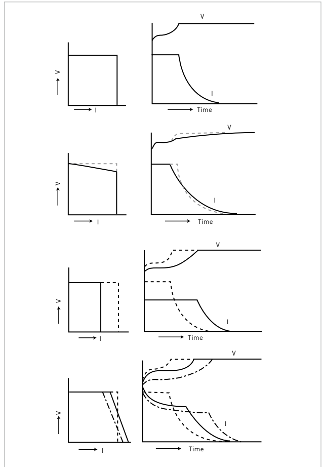
Fig. 7 Output V-I characteristics of the constant voltage charger vs. charging pattern of the battery
