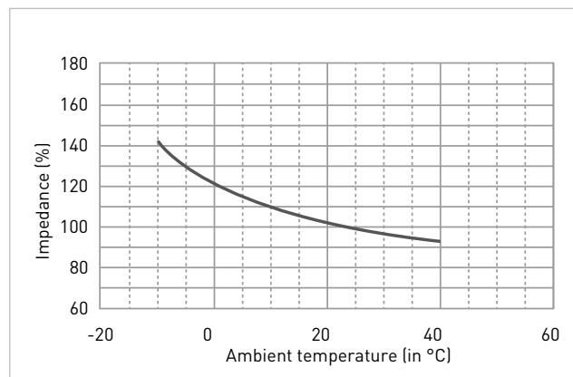
Fig. 7 Relationship between impedance and temperature
