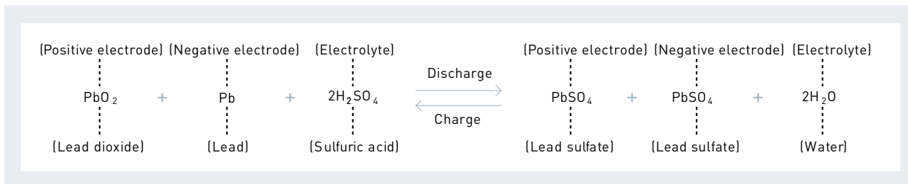
Fig. 6 Charge / discharge chemical equation
