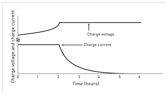
Fig. 1 Constant voltage constant-current charge characteristics
