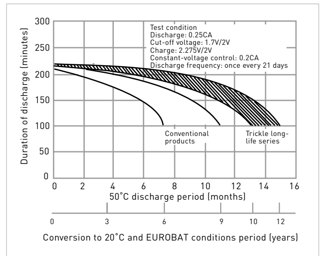
Fig. 10 Influence of temperature on trickle life
