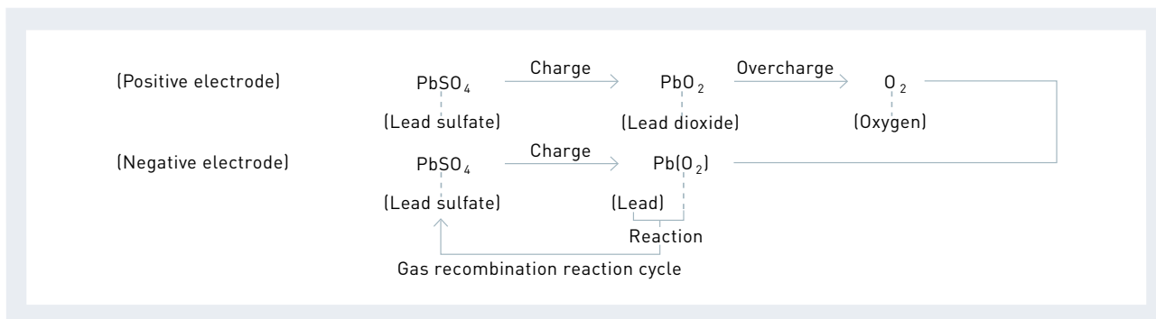
Fig. 7 Recombination chemical equation
