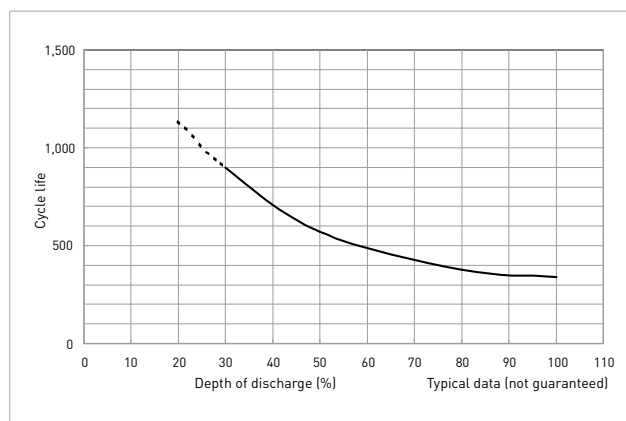
Fig. 8 Cycle life vs. depth of discharge (cyclic models)
