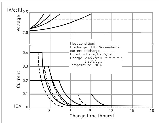
Fig. 1 Constant-voltage charge characteristics by current (example)
