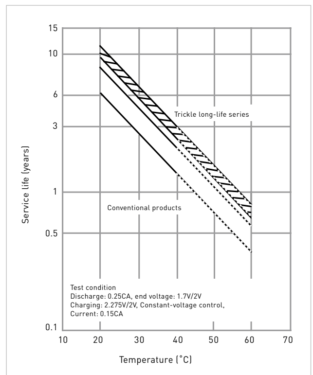
Fig. 10 Influence of temperature on trickle life
