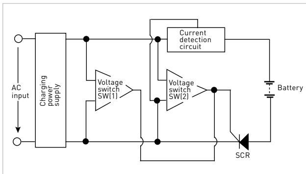
Fig. 3 Diagram of the two-step constant voltage control charger
