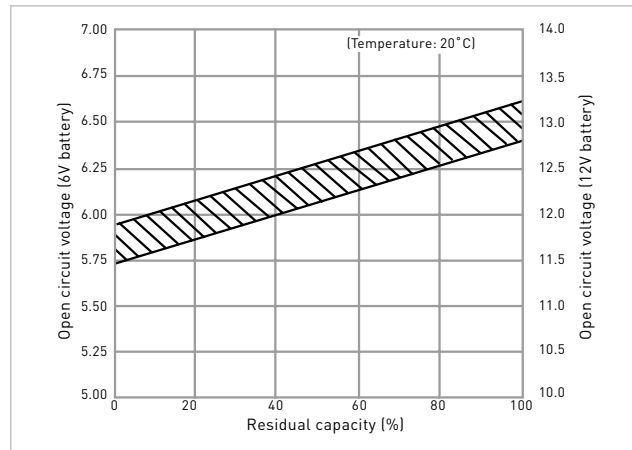
Fig. 5 Open circuit voltage vs. residual capacity 20^{\circ}\text{C}
