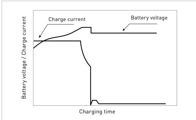
Fig. 3 Diagram of the two-step constant voltage control charger
