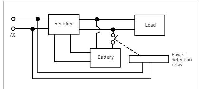
Fig. 4 Trickle charge system model
