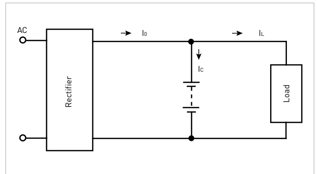
Fig. 5 Float charge system model
