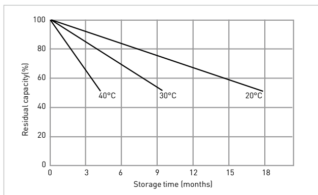
Fig. 4 Residual capacity test result
